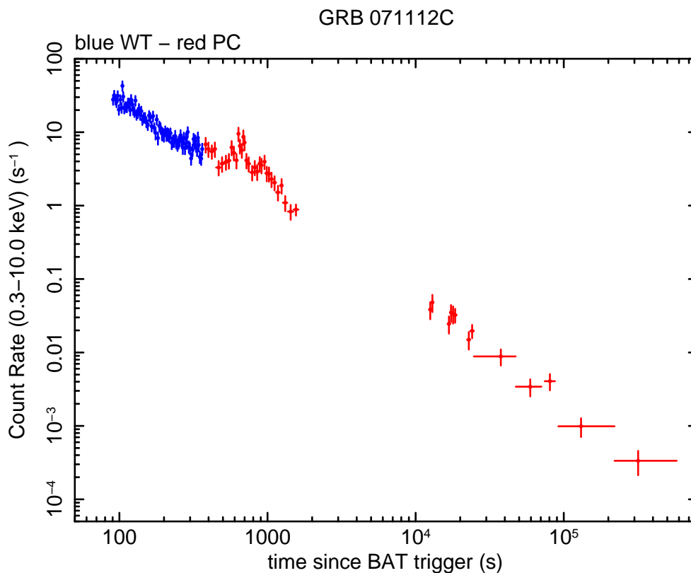
Figure 2: XRT Lightcurve. Count s^{-1} in the 0.3-10 keV band: Window Timing mode (blue), Photon Counting mode (red). The approximate conversion is 1 \text{ count } s^{-1} \sim 4.5 \times 10^{-11} \text{ erg cm}^{-2} s^{-1} .
